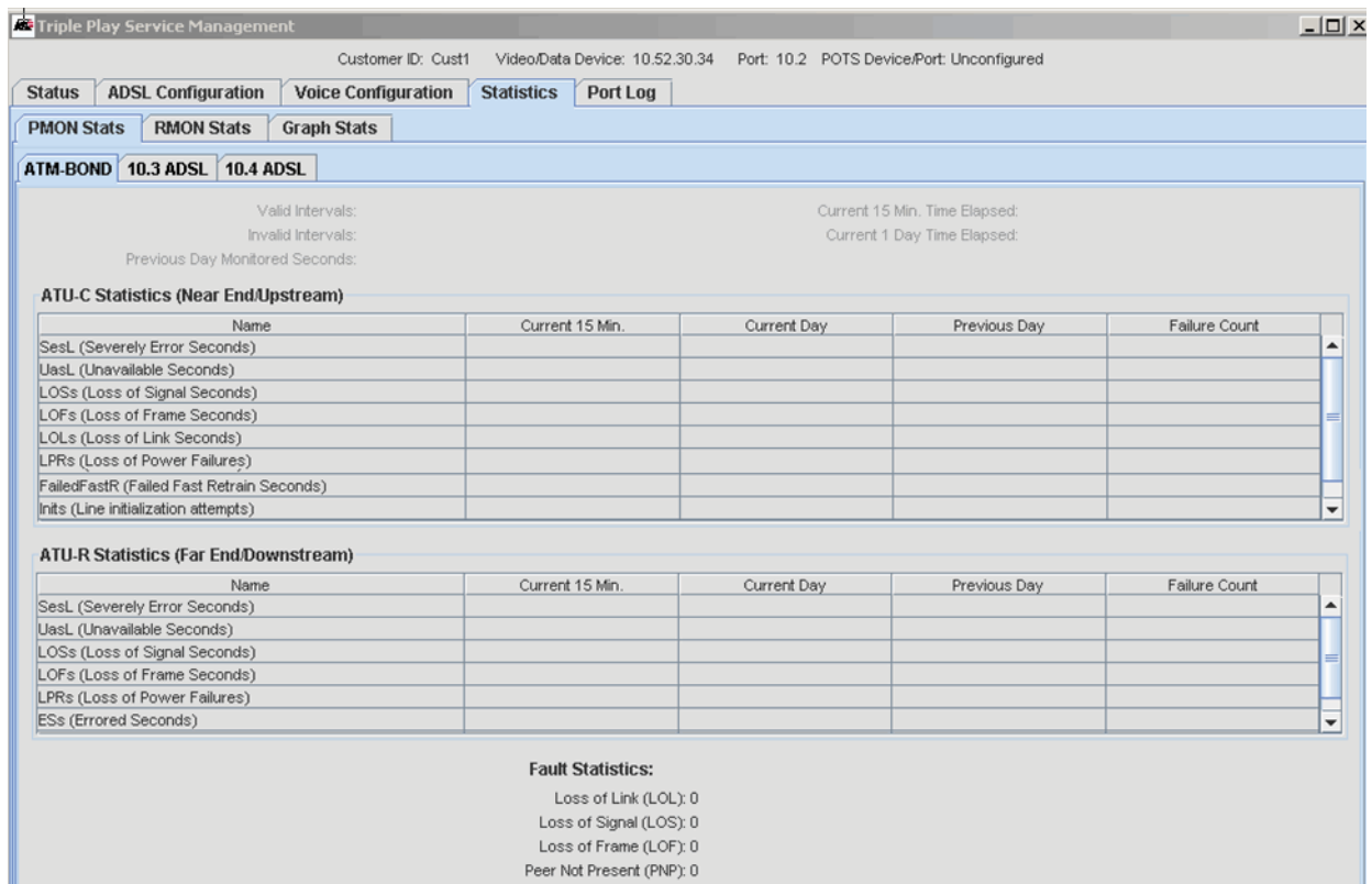
FIGURE 5-161 PMON Stats - ADSL Bonding
