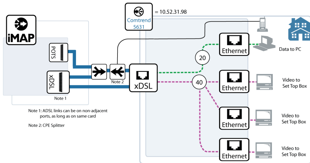
FIGURE 5-222 Comtrend Configuration (Bonded ADSL)
