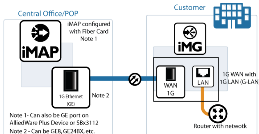
FIGURE 7-120 Example iMG7x6MOD Configuration (Simplified)
