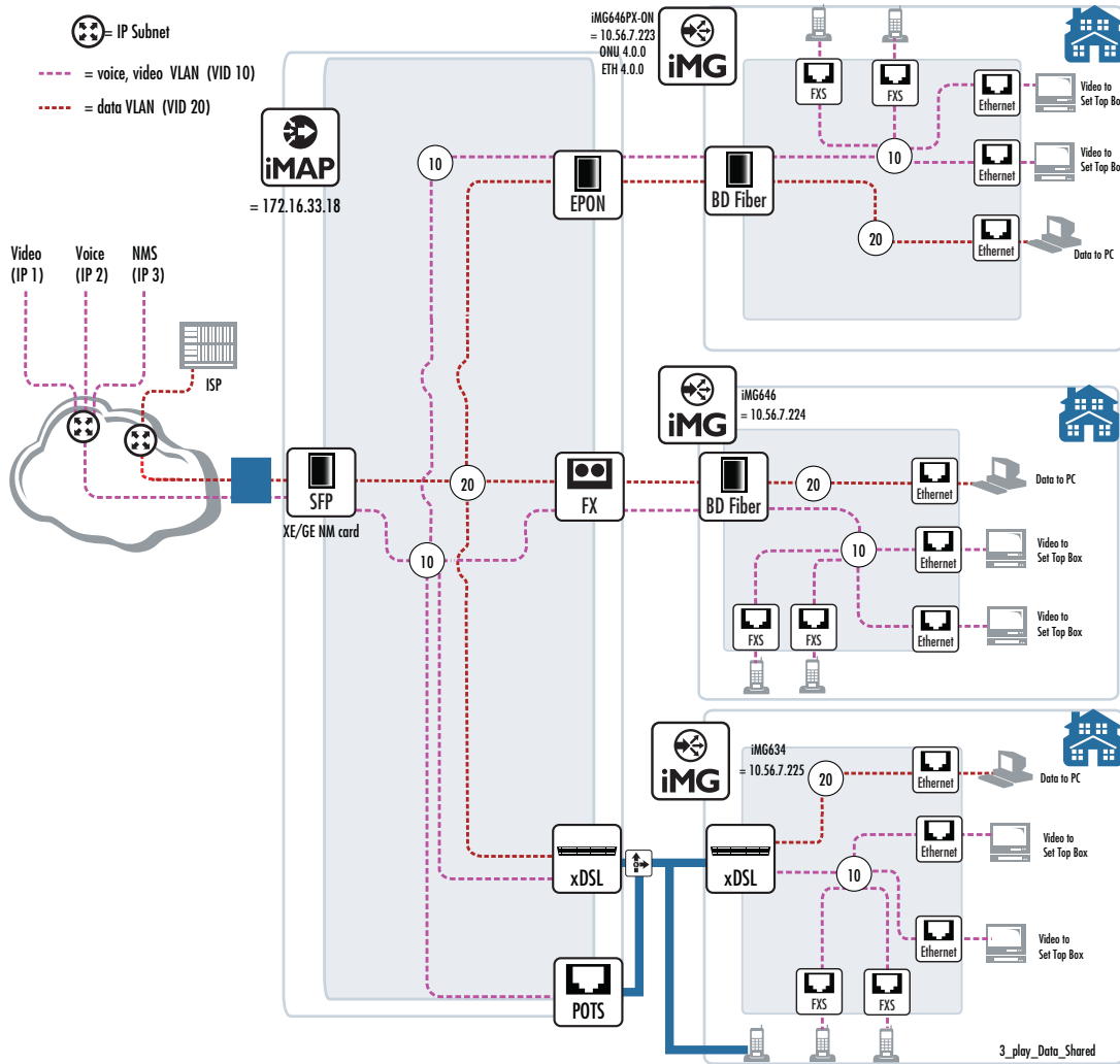
FIGURE 7-173 Multi-service (Video, Video) VLAN (Configuration 2)
