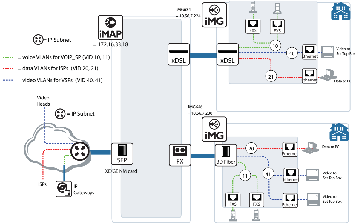
FIGURE 7-3 Multiple ISP Configuration
