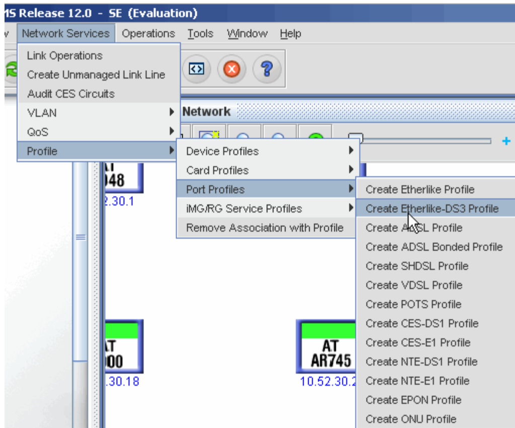
FIGURE 6-69 Profile for DS3 SFP
