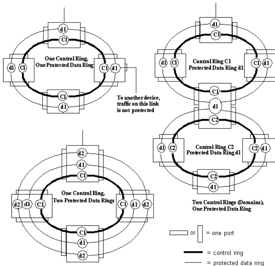
FIGURE 6-107 Example Ring Topologies
