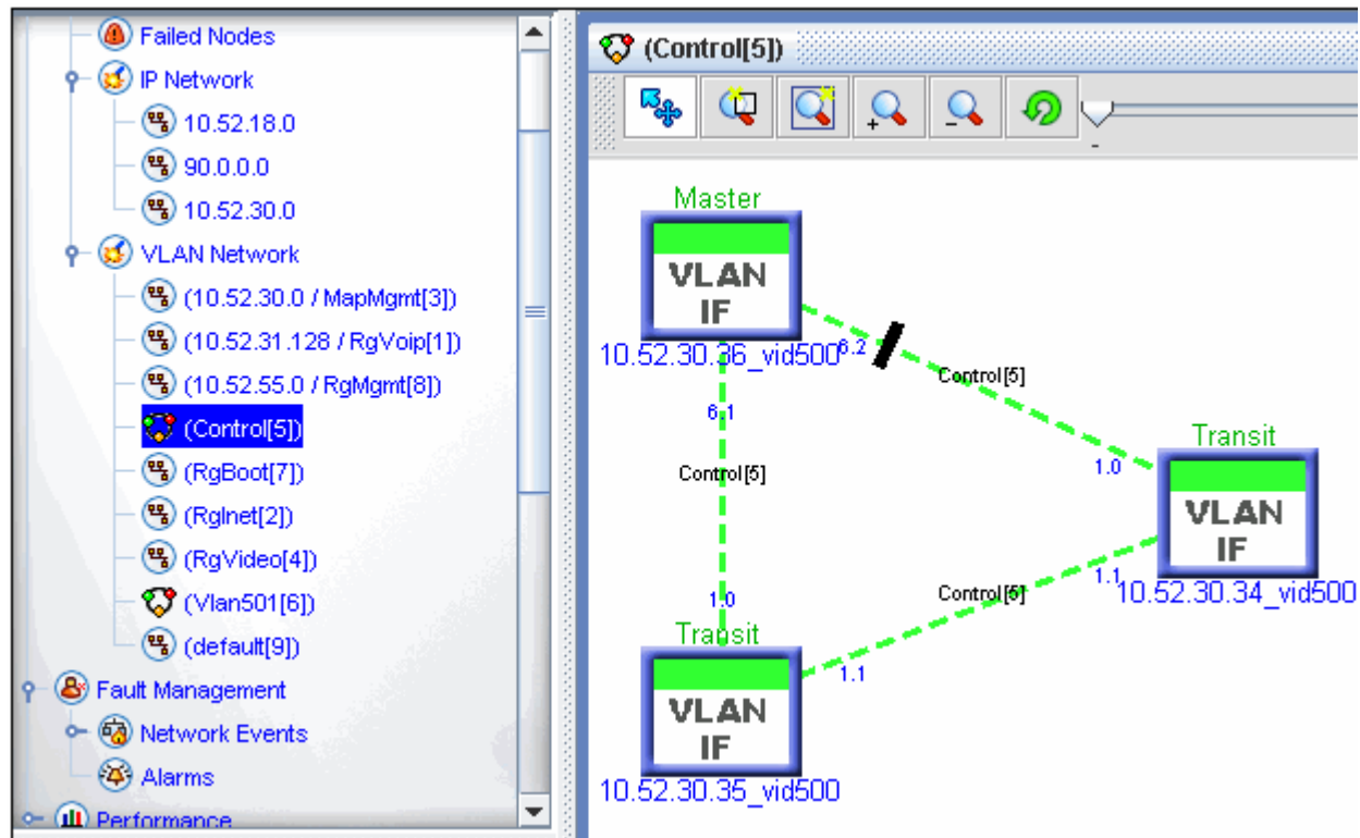
FIGURE 6-236 EPSR - Control VLAN over Physical Links
