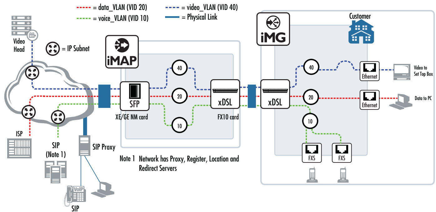
FIGURE 7-74 Configuration 5 - VoIP using SIP
