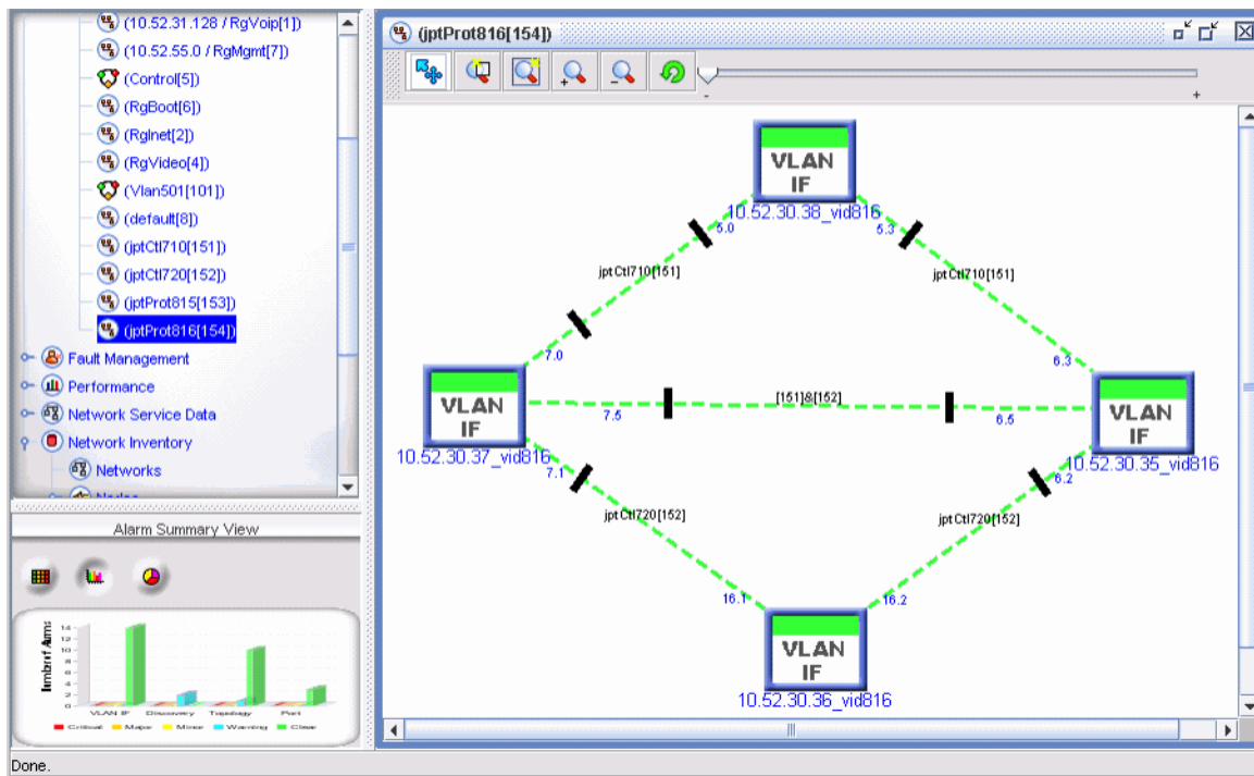
FIGURE 6-170 Protected VLAN across Multiple EPS Control VLANs (816)
