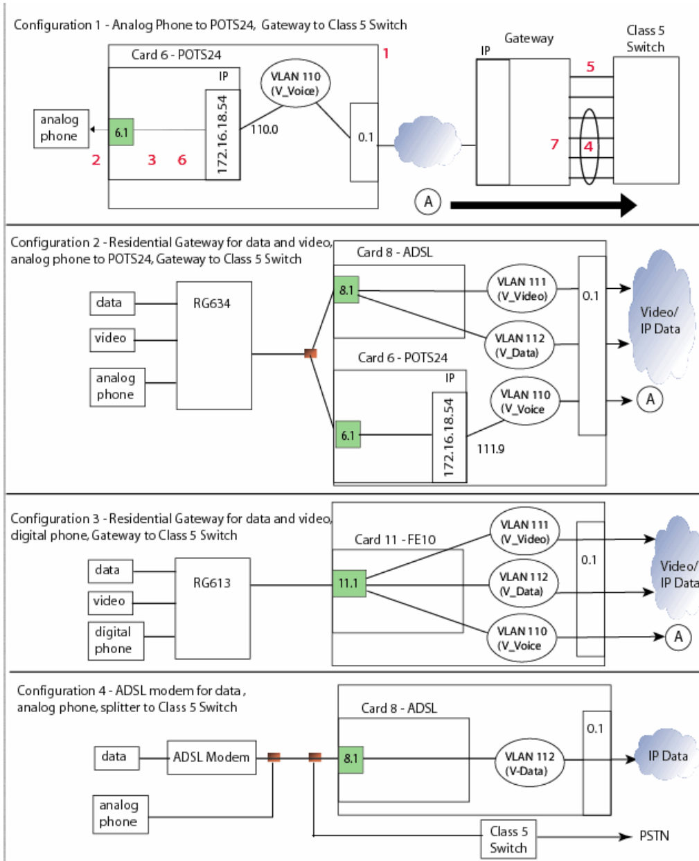
FIGURE 6-173 Four Example Configurations for Triple Play
