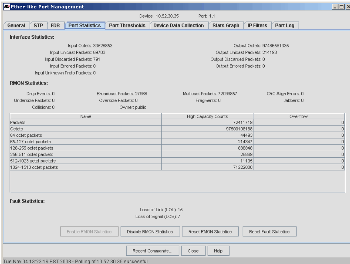
FIGURE 5-143 Ether like Port Management Window - Port Statistics Tab
