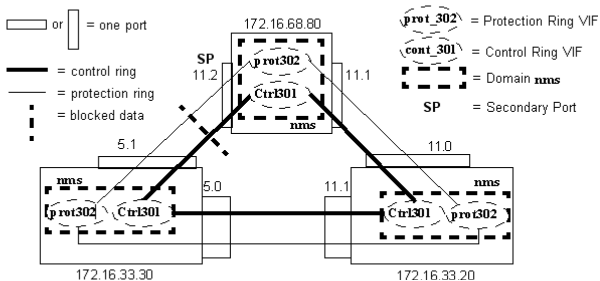
FIGURE 6-117 Example Ring Topology - Physical/Logical
