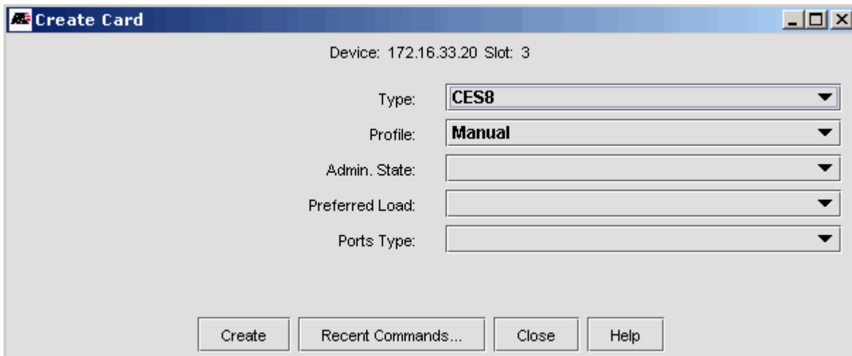
FIGURE 5-108 Create Card Window for CES8 Card
