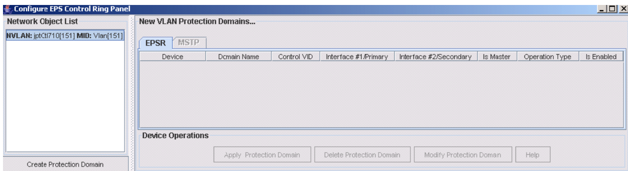
FIGURE 6-145 Configure EPS Control Ring Panel
