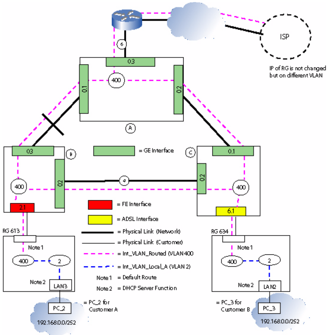
FIGURE 7-35 Internet - Routed Configuration
