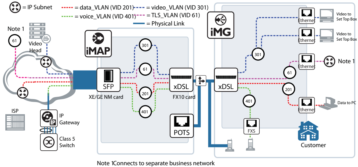
FIGURE 7-55 Example Configuration 1 - Internet Routed/NAT, Video Proxy, Lifeline POTS, TLS
