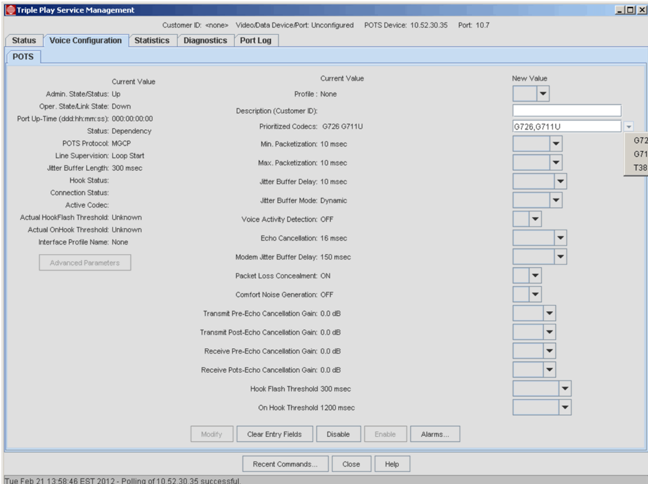
FIGURE 5-168 Example POTS24 Voice Configuration Tab - POTS (SIP Protocol)
