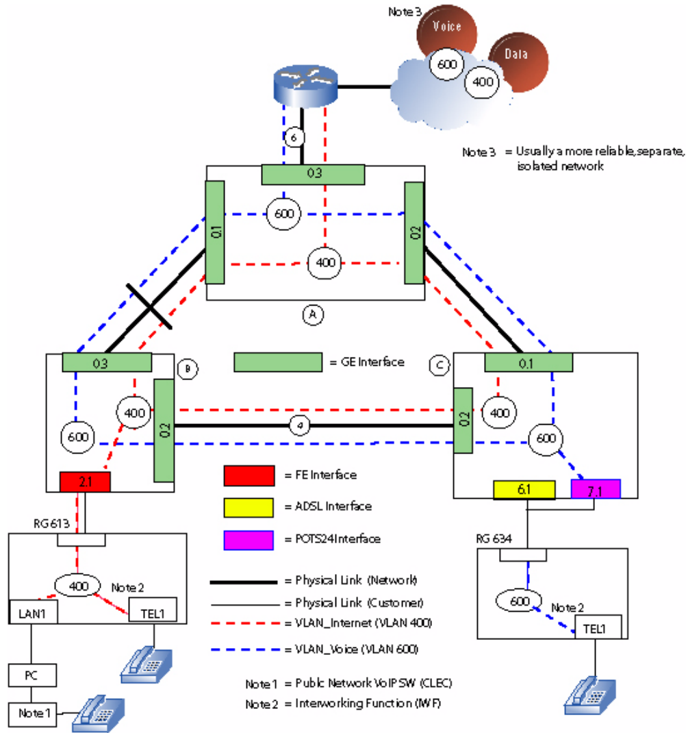
FIGURE 7-47 Voice - Public and Private Configuration
