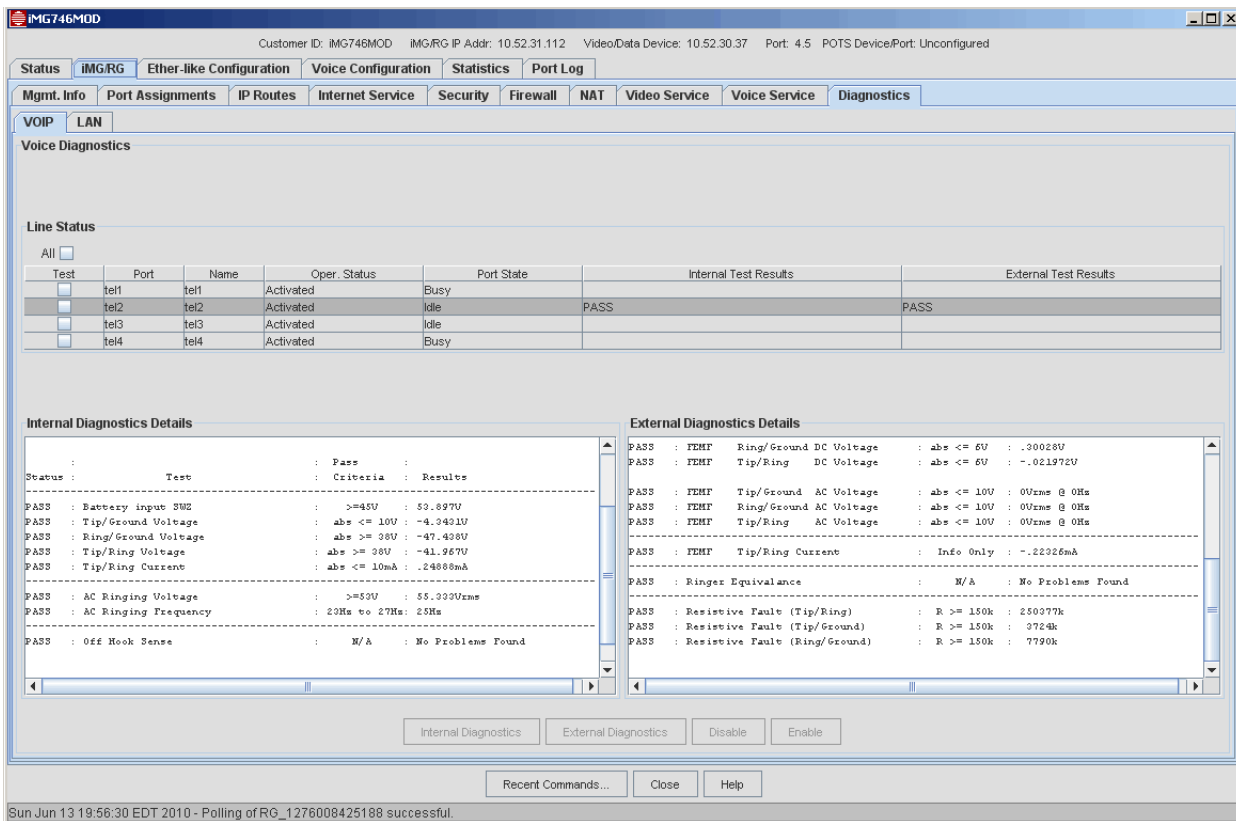
FIGURE 7-212 GR909 Test Results
