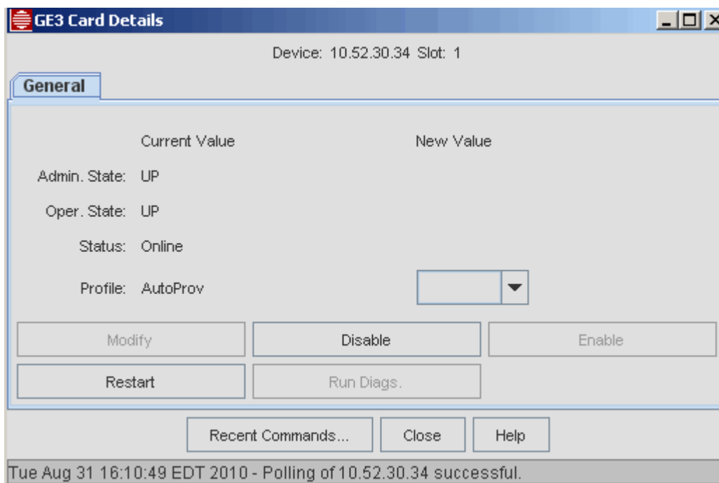
FIGURE 5-109 GE3 Card Details
