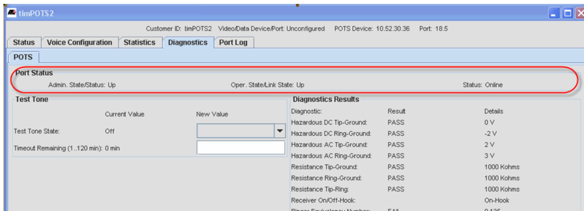
FIGURE 5-170 POTS24 Diagnostics Tab - Port Status
