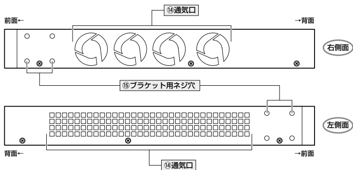
AT-FS980M/28DP
