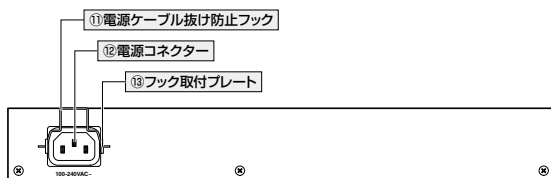
AT-FS980M/9
