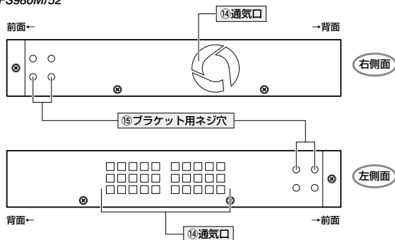
AT-FS980M/28PS-52PS
