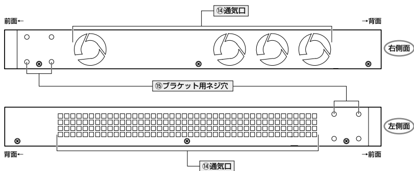
AT-FS980M/28DP
