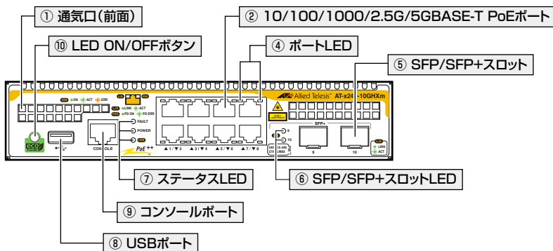
AT-x240-10GHXm
