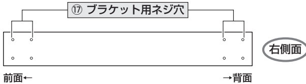
AT-x510-28GPX / AT-x510-52GPX
