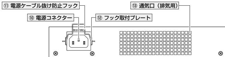
AT-XS916MXS / AT-XS916MXT
