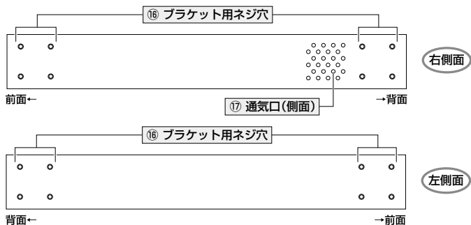
AT-GS980M/52
